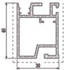
Tapa final barra End cap for rack
